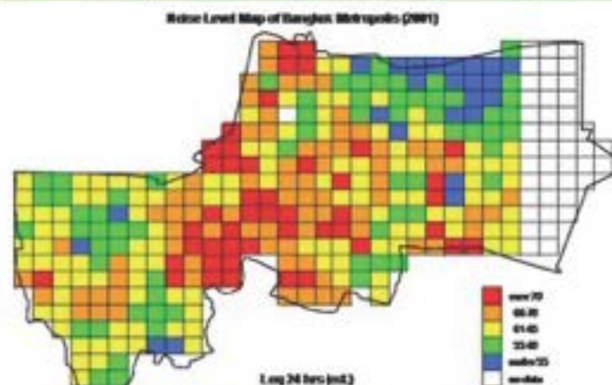
Bangkok Noise Mapping in 2001
