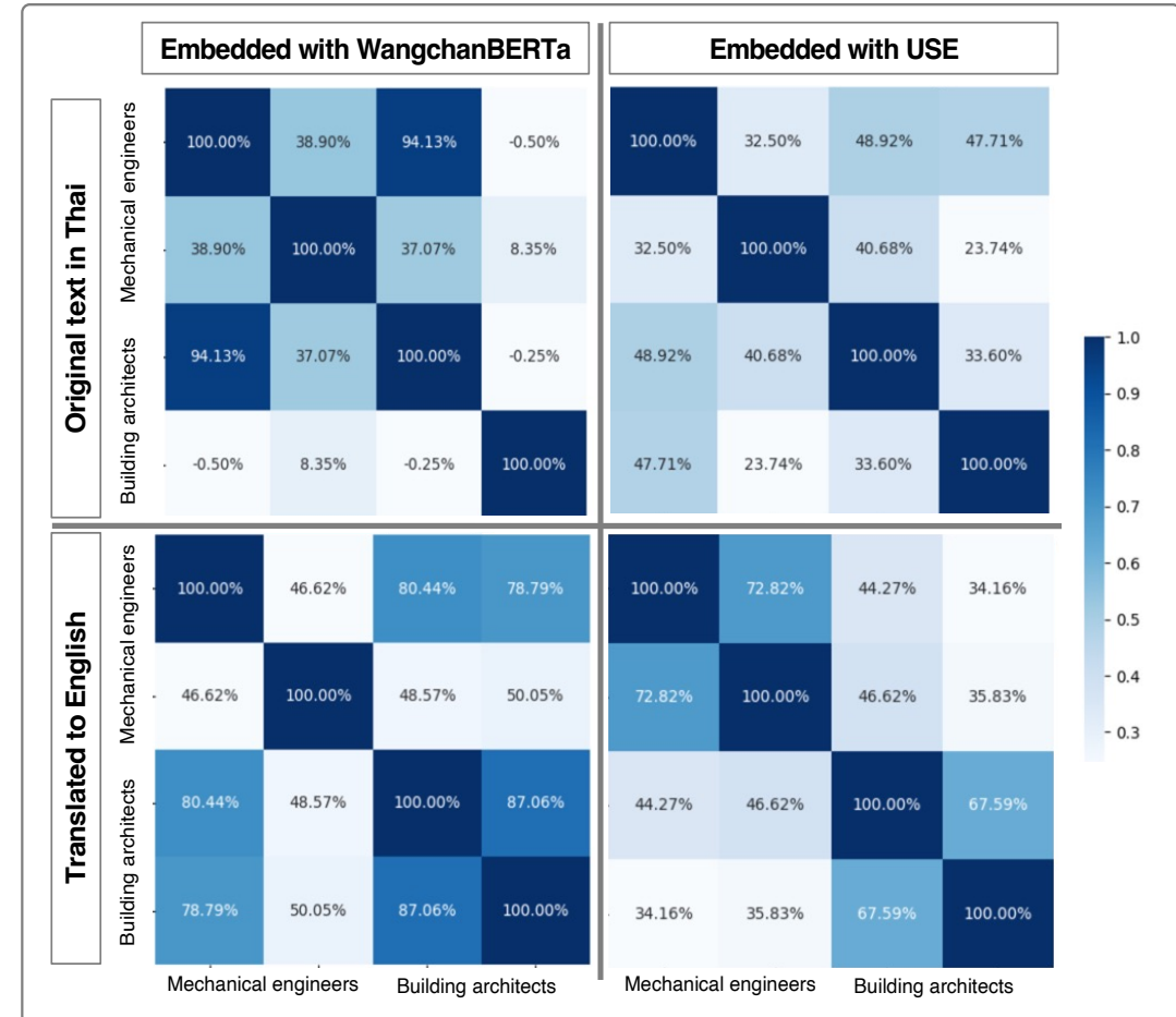
Figure 1: Cosine Similarity Matrices at Stage One
